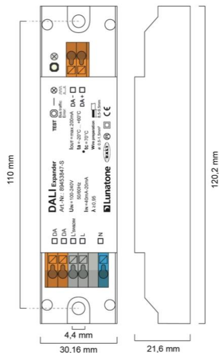
dimensions DALI Expander (S-type) Art.Nr.: 89453847-S
