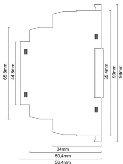
dimensions DALI-Expander (HS-type)
