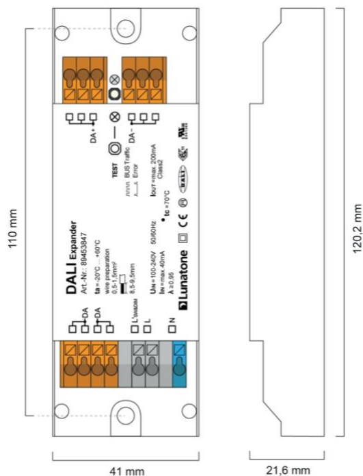
dimensions DALI Expander Art.Nr.: 89453847
