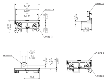
DIRECT MOUNTING
