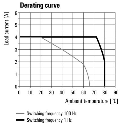
Deratingkurve
