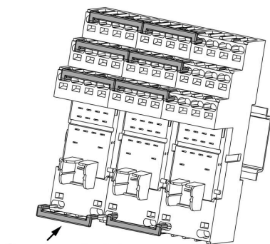
Plug cross connection direct into wire-connection opening
