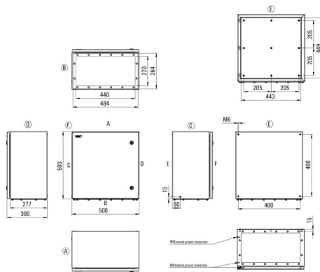
VIEW WITHOUT COVER, SEAL AND SCREW
