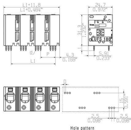
Hole pattern
