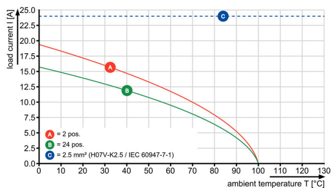
BLZP 5.08/.../225 - SL 5.08/.../90
