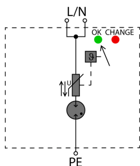
Schematic circuit diagram
