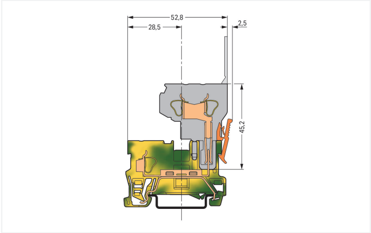
Ground carrier terminal block
