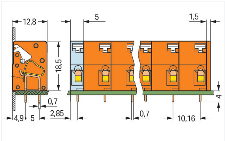
Misure in mm Total length = (pole no. – 1) x pin spacing + 5 mm + 1.5 mm
