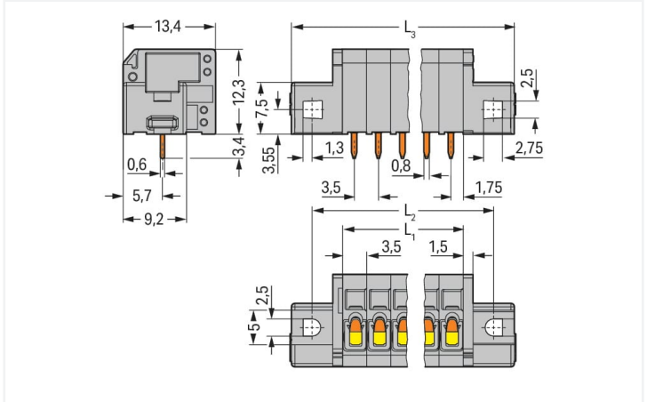
Misure in mm L1 = pole no. x pin spacing L2 = L1 + 8.8 mm L3 = L1 + 14.8 mm
