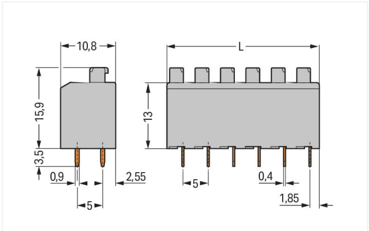
Misure in mm L (2-pole): 10 mm, L (3-pole): 15 mm L (4-pole): 20 mm, L (6-pole): 30 mm L (7-pole): 35 mm
