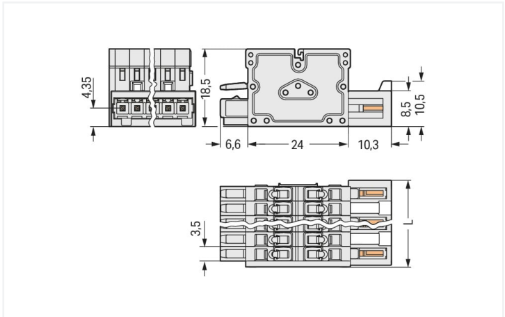
Misure in mm L = (pole no. – 1) x pin spacing + 5.9 mm + 0.45 mm
