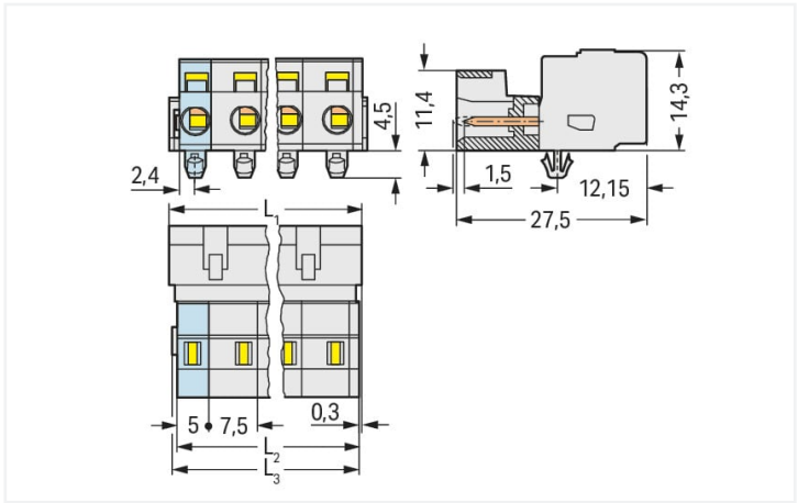
Misure in mm L1 = (pole no. - 1) x pin spacing + 8.2 mm L2 = L1 - 1.7 mm L3 = L1 - 1.2 mm
