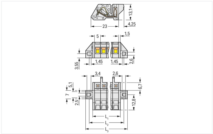
Misure in mm L1 = (pole no. x pin spacing) + 3 mm L2 = (pole no. x pin spacing) + 8.8 mm L3 = (pole no. x pin spacing) + 14.8 mm
