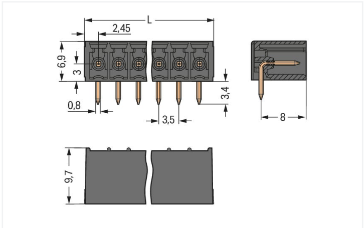
Misure in mm L = (pole no. – 1) x pin spacing + 4.9 mm
