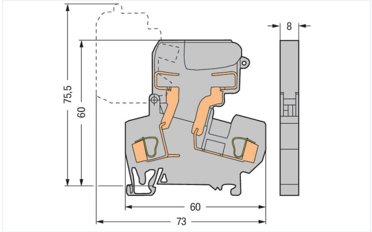
Misure in mm Fused disconnect terminal block with a pivoting fuse holder, for (5 x 20) mm glass cartridge fuse, without blown fuse indication (281-611)
