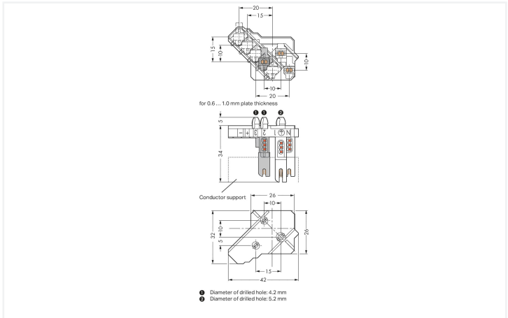
Misure in mm 1) Diameter of drilled hole: 4.2 mm 2) Diameter of drilled hole: 5.2 mm
