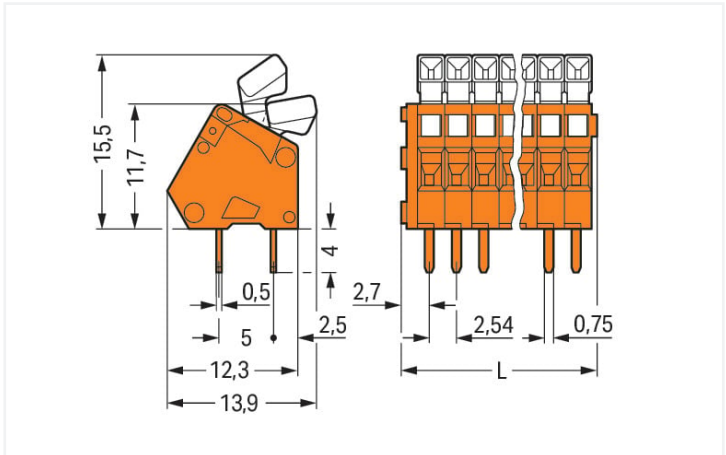
Misure in mm L = (pole no. x pin spacing) + 2.3 mm
