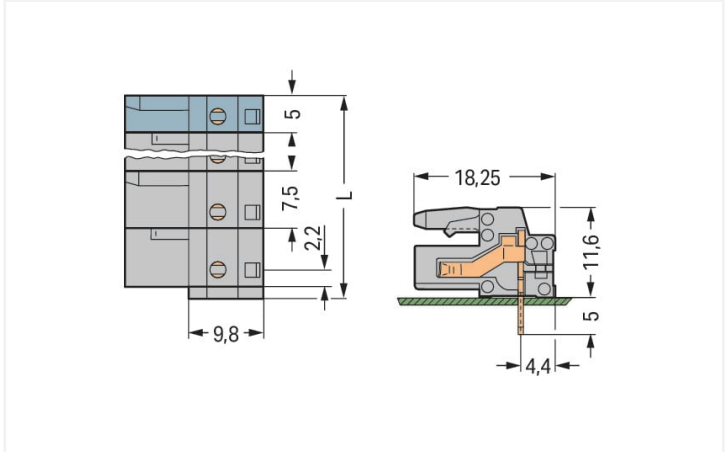
Misure in mm L = (pole no. – 1) x pin spacing + 5 mm + 1.5 mm Distance to first solder pin: 2.2 mm 2- to 3-pole female connectors – one latch only
