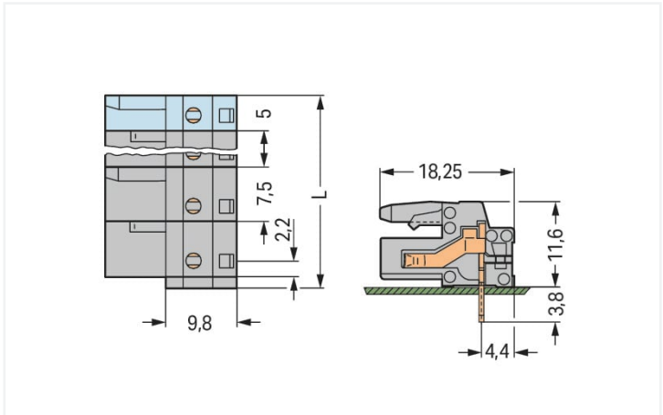
Misure in mm L = (pole no. - 1) x pin spacing + 5 mm + 1.5 mm 2- to 3-pole female connectors – one latch only
