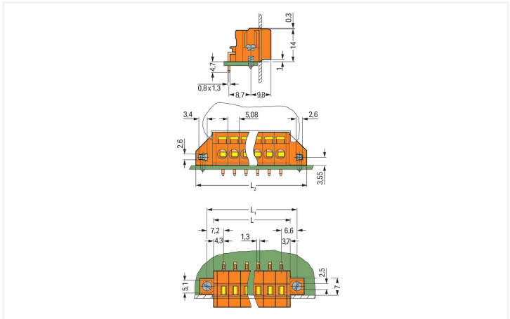
Misure in mm L = (pole no. x pin spacing) + 3 mm L1 = L + 5.8 mm L2 = L1 + 6.4 mm
