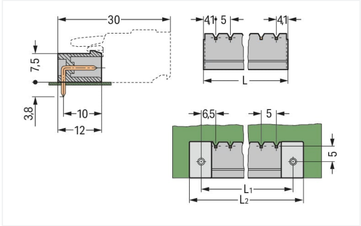
Misure in mm L = (pole no. – 1) x pin spacing + 8.2 mm L1 = L + 5 mm L2 = L1 + 7.4 mm
