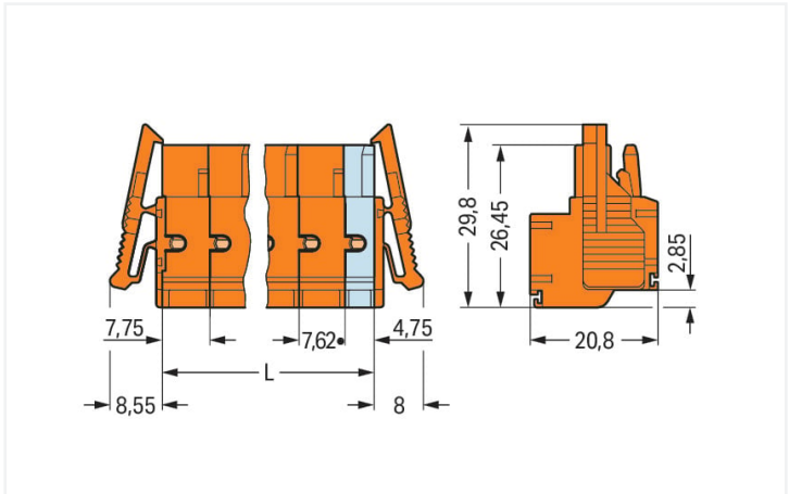
Misure in mm L = (pole no. – 2) x pin spacing + 12.5 mm 2- to 3-pole female connectors – one latch only
