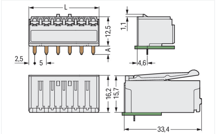
Misure in mm L = pole no. x pin spacing A = 3.6 mm THT solder pin A = 2.4 mm THR solder pin
