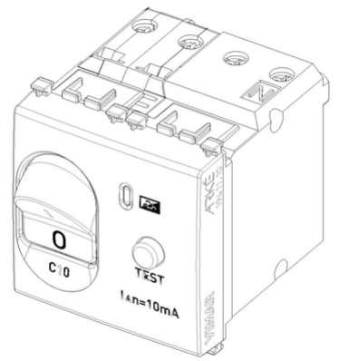
Vista 3D
