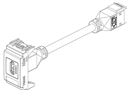
Vista 3D
