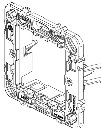
Vista 3D
