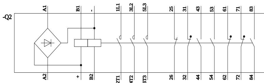
3TF(68,69)33-(1Q,8Q)xx
