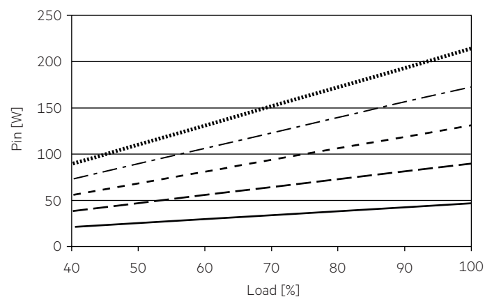
4.5.3 Input power vs. load 277 V, 60 Hz
