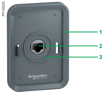
Remote-mounting kit VW3A1114 (front view)
