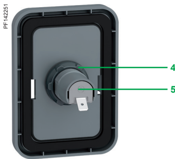
Remote-mounting kit VW3A1114 (rear view)
