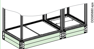
Side-by-side combination of two cubicles with a plinth.
