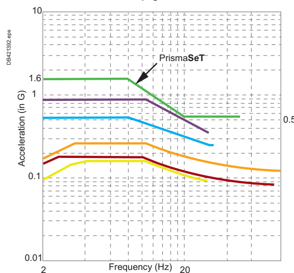
Compare PrismaSeT G Switchboards Performances with seismic Standard Damping % - vertical
