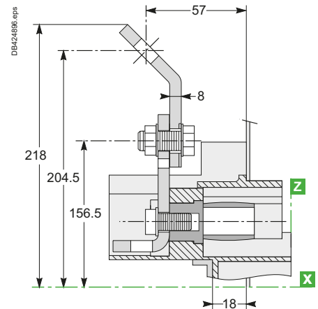
NSX400/630
