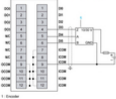
Incremental encoder connection with push-pull at outputs
