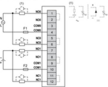
2-wire connection (AC and DC)
