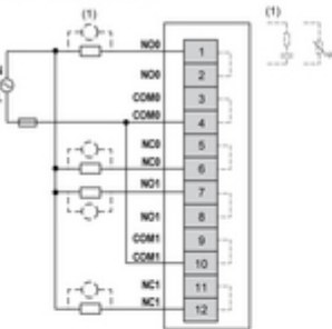
2-wire connection (AC)
