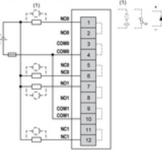
2-wire connection (DC)
