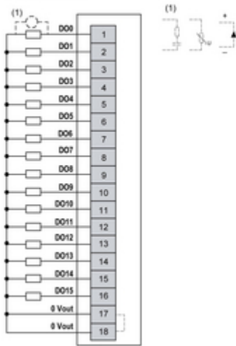
2-wire connection
