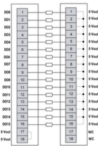
2-wire connection (with common module)
