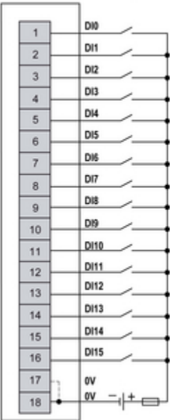
1-wire connection (with external power supply)
