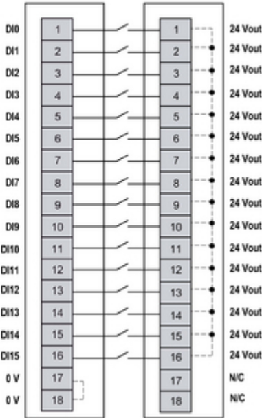
1-wire connection (with common module)
