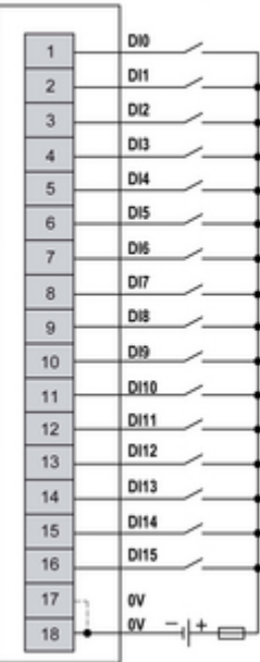
1-wire connection (with external power supply)
