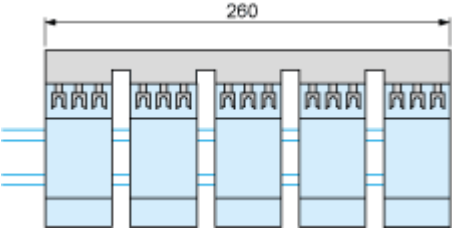
Set of busbars GV2G554
