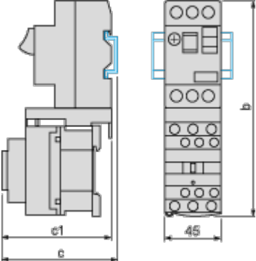
GV2AF3 Combination GV2ME + TeSys d contactor
