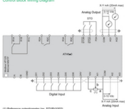
Control Block Wiring Diagram
