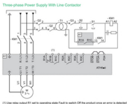
Control Block Wiring Diagram
