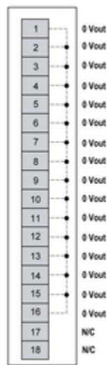
Wiring diagram for the NTSPCM0016H
