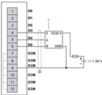
Incremental encoder connection
