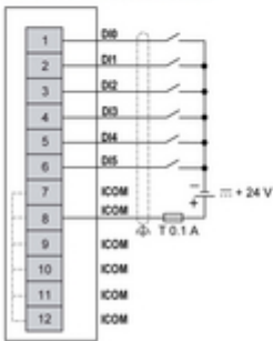
2-wire source input connection
