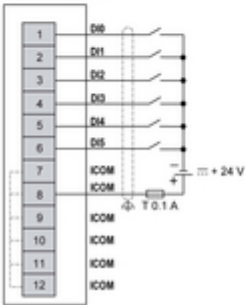
2-wire source input connection
