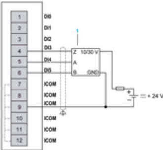
Incremental encoder connection
