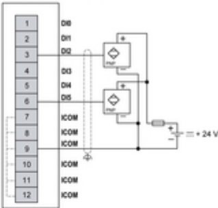
3-wire input connection
