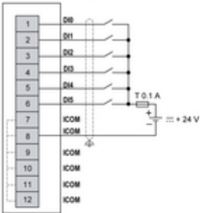
2-wire sink input connection
