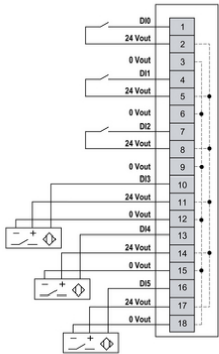
2-wire or 3-wire connection
