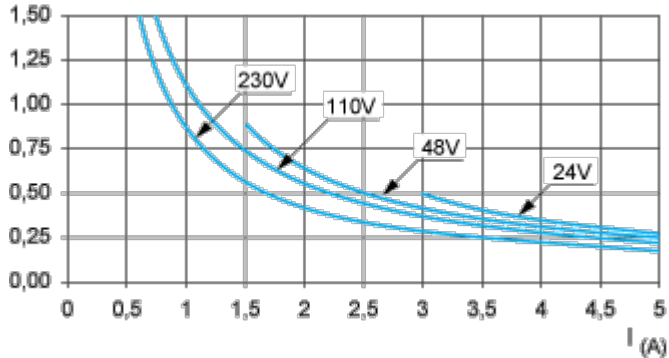
Curve AC15
