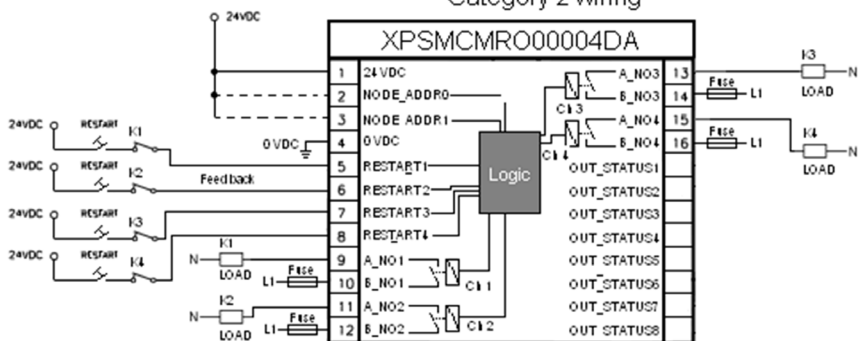
Category 2 wiring
