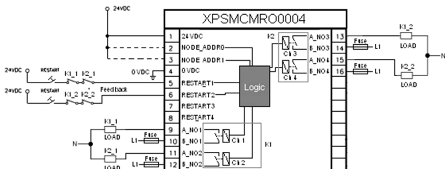
Category 4 wiring
