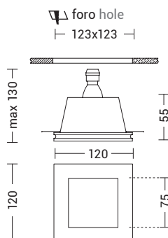
modulo COB LED COB LED unit
