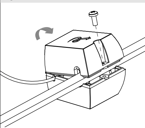
Chiusura del box isolante sul morsetto Closing of insulation box with connector inside
